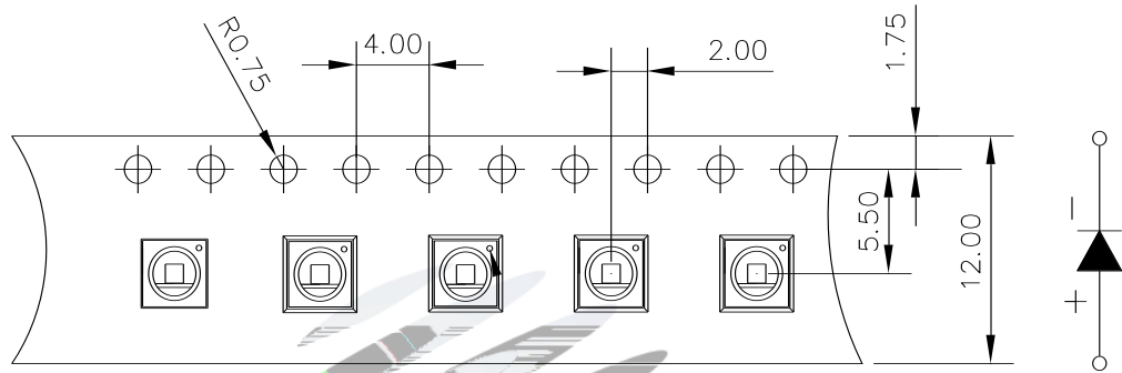
Fig.2-1 Carrier Tape Dimension 载带尺寸
