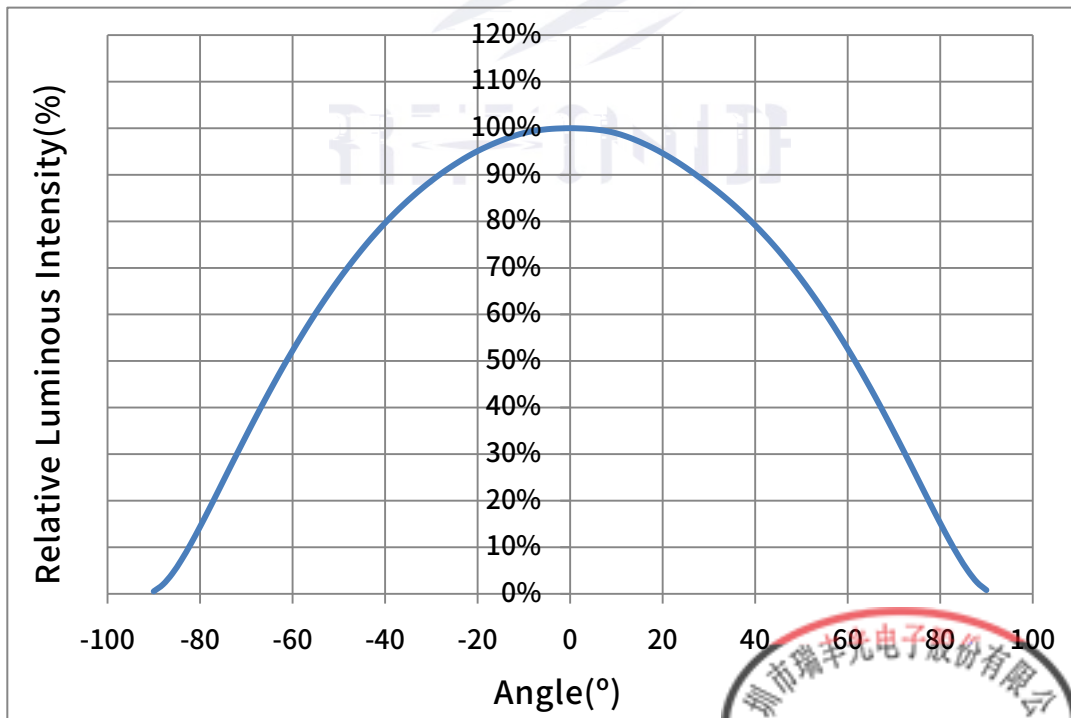
Fig. 1-12 Radiation diagram
