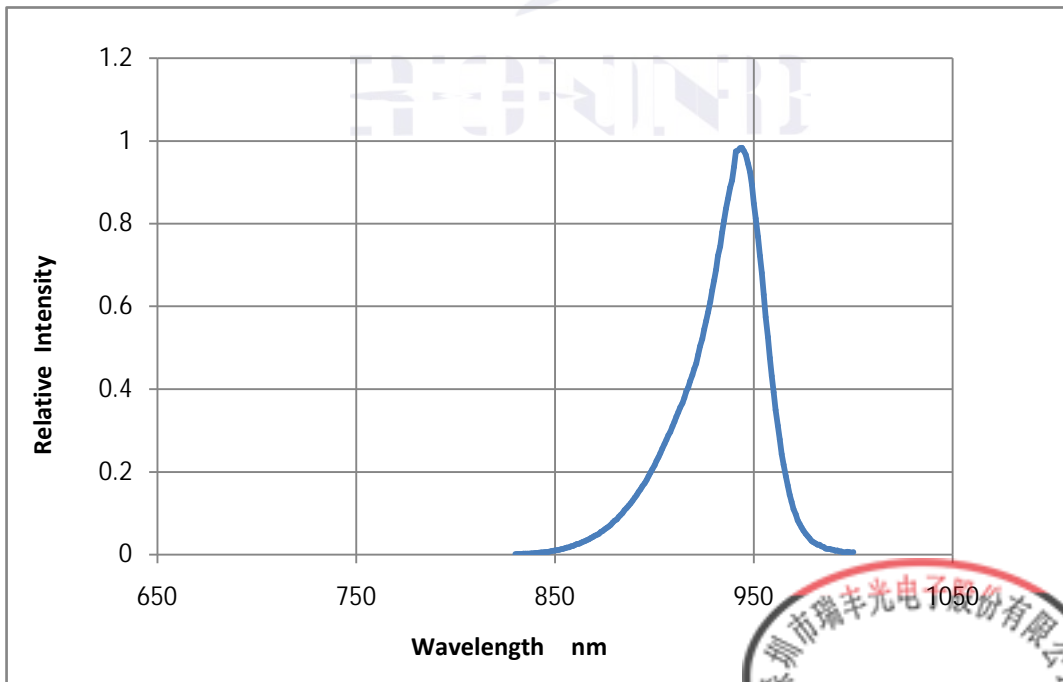
Fig. 1-14 Spectrum Distribution
