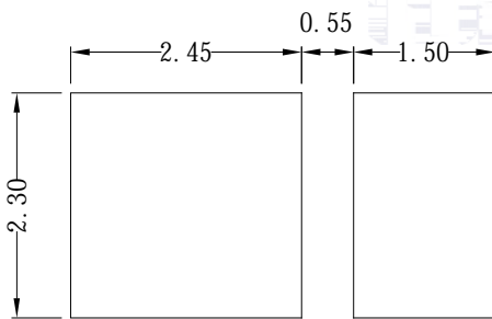
Fig.1-5 Soldering Patterns
