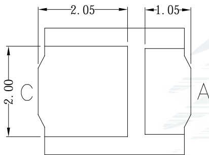
Fig.1-3 Bottom View
