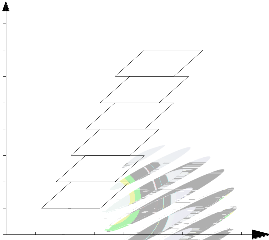
Fig. 1-6 The C.I.E Chromaticity Diagram CIE
