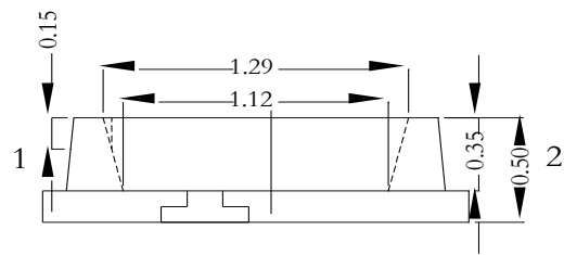
Fig.1-2 Side view
