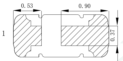
Fig.1-3 Bottom view
