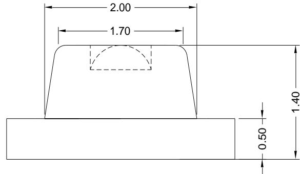
Fig.1-2 Side view
