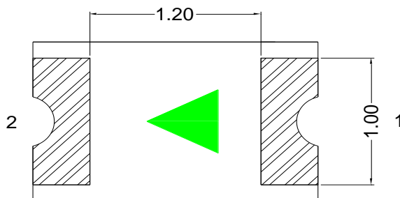
Fig.1-2 Bottom view
