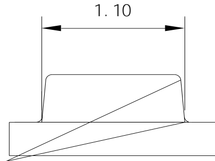
Fig.1-2 Side view
