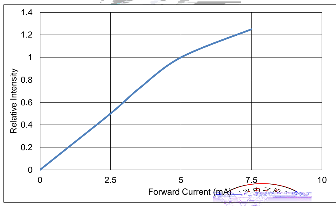
Fig 1-7 Forward Current Vs Relative Intensity
