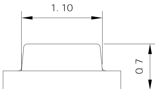
Fig.1-2 Side view
