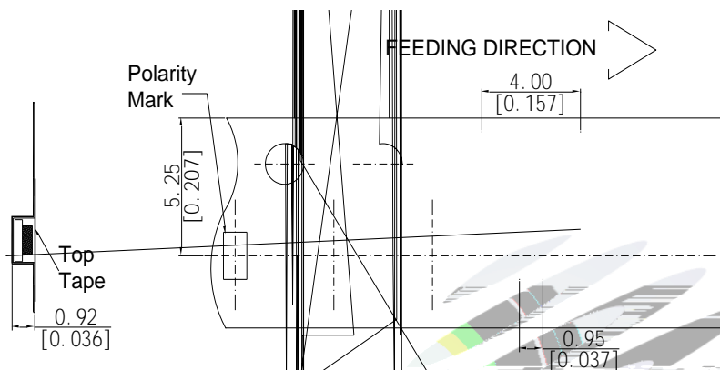
Fig.2-1 Carrier Tape Dimension
