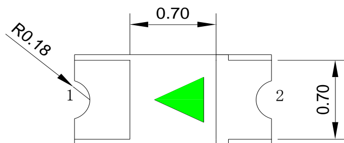
Fig.1-2 Bottom view
