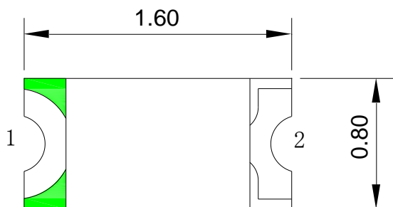
Fig.1-1 Top view
