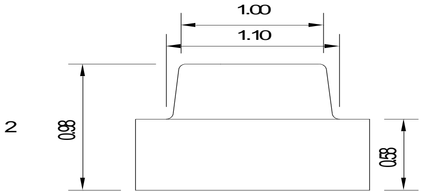
Fig.1-2 Side view
