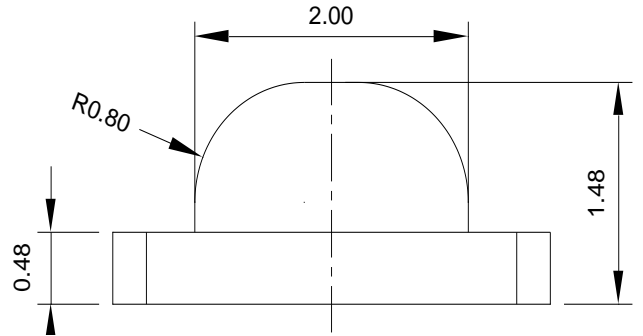
Fig.1-2 Side view
