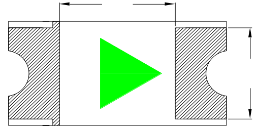
Fig.1-1 Top view
