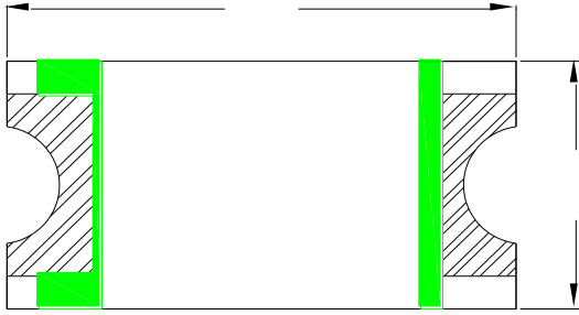
Fig.1-2 Bottom view
