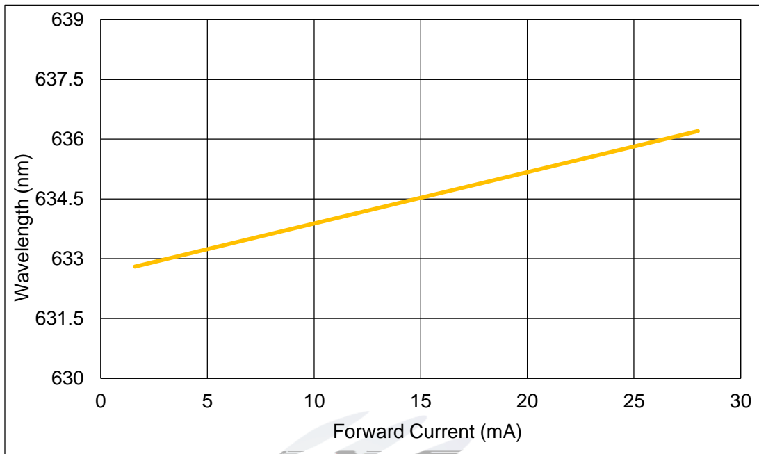
Fig.1-10 Forward Current Vs Dominate Wavelength ( T_a=25^\circ\text{C} )
