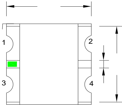
Fig.1-1 Top view
