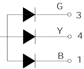
Fig.1-4 Polarity
