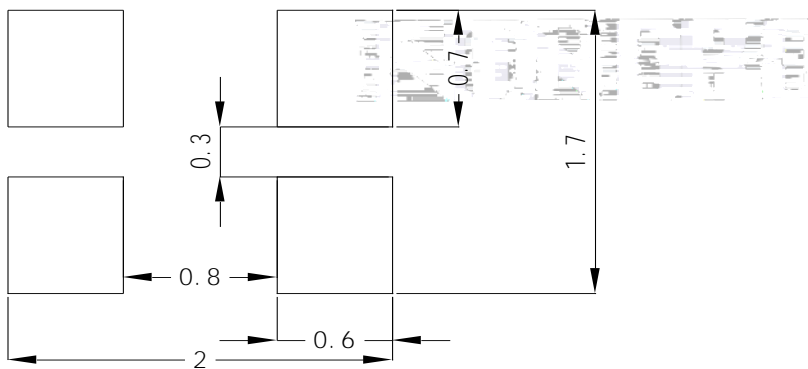
Fig.1-5 Soldering patterns
