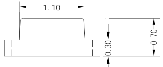
Fig.1-2 Side view
