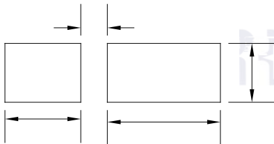
Fig. 1-5 Soldering Patterns
