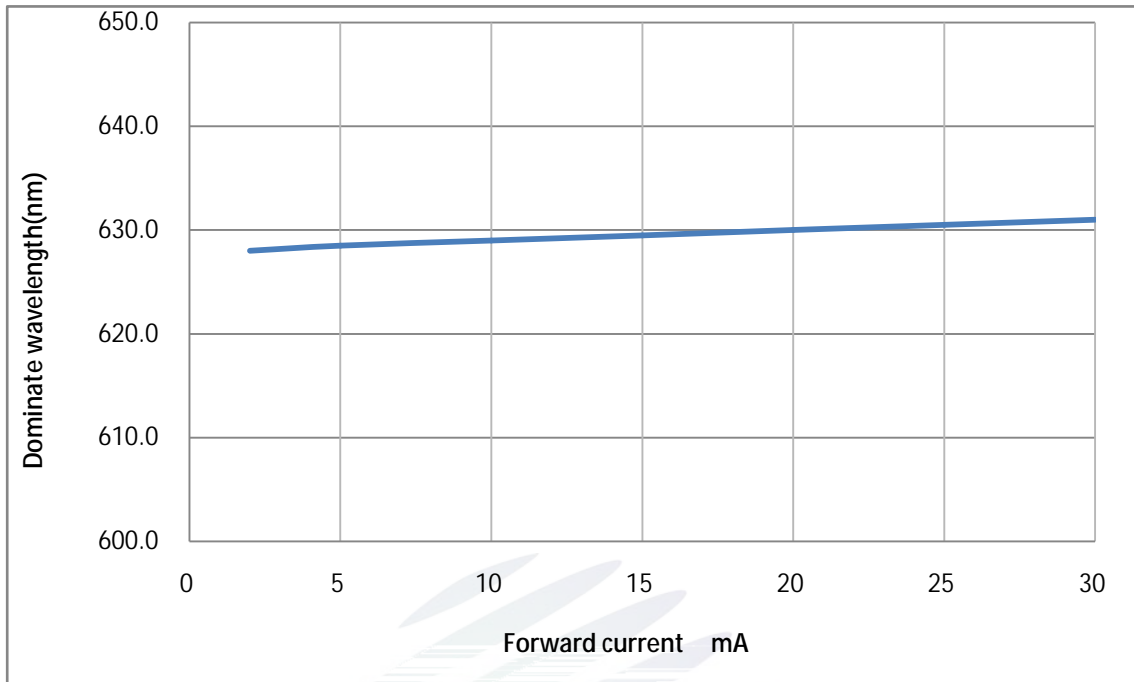
Fig. 1-13 Forward Current vs. Color Shift (Ts=25°C) (Ts=25°C)
