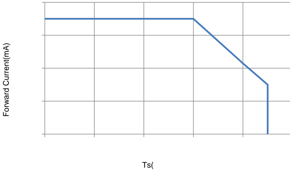
Fig.4-Ts Temperature VS. Forward Current
