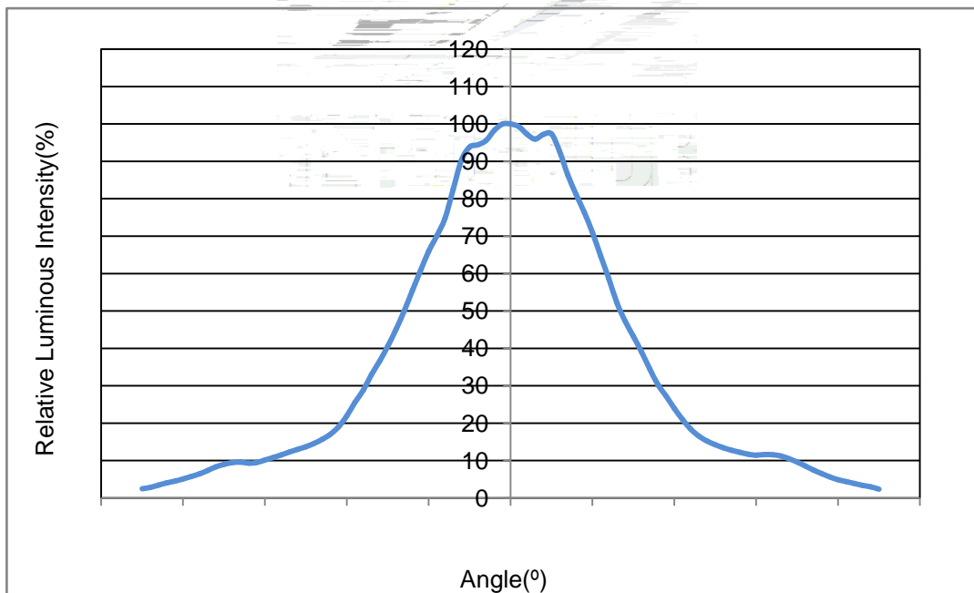
Fig.6- Radiation Diagram
