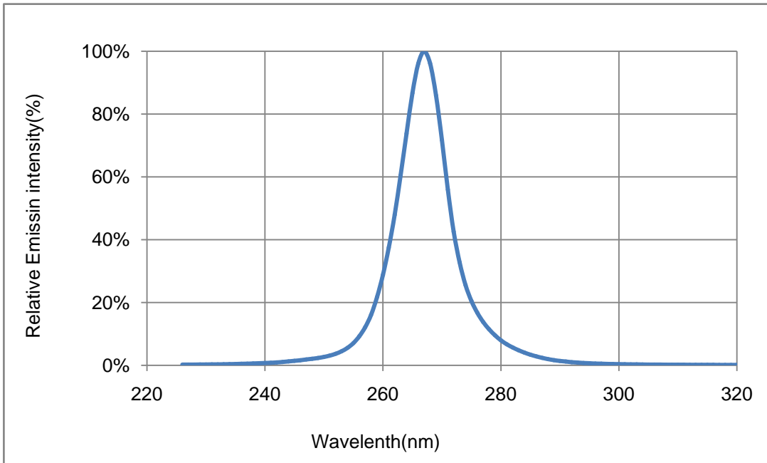
Fig.5-Spectrum Distribution
