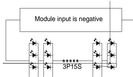
Fig.2-2ED Module connection
