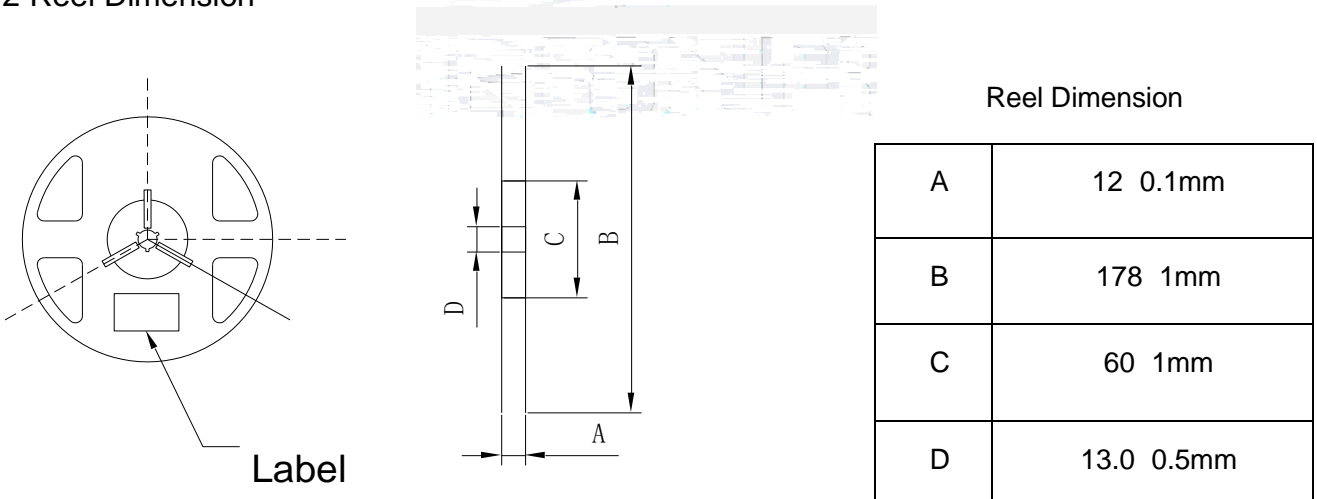
Fig.2-2 Reel Dimension
