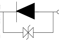
Fig.1-4 Polarity
