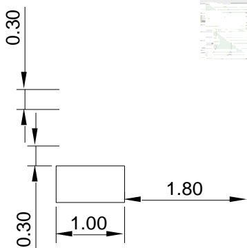
Fig.1-5 Soldering patterns 堆焊焊盘
