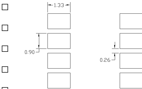
Fig.1-3 Bottom view
