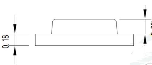
Fig.1-3 Side view
