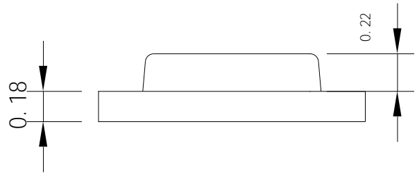
Fig.1-2 Side view
