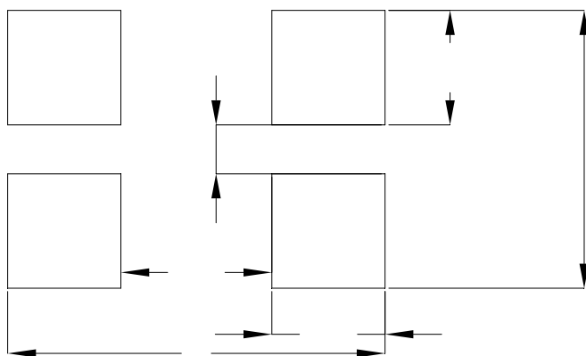
Fig.1-5 Soldering patterns
