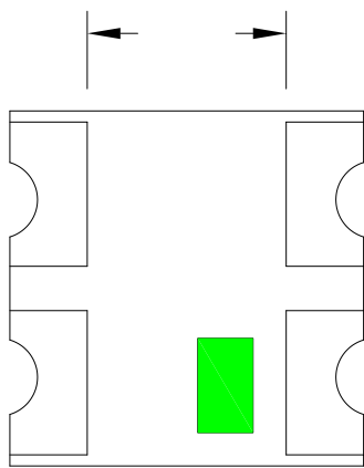
Fig.1-3 Bottom view
