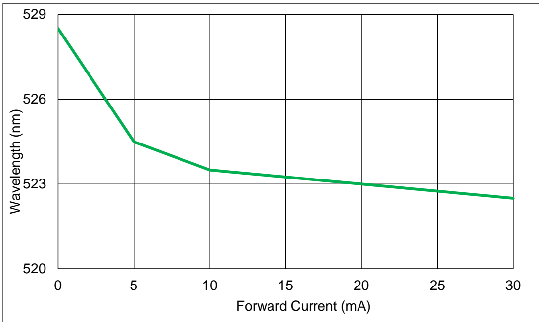
Fig.1-12 Forward Current Vs Dominate Wavelength (Ta=25°C) 正向电流与主波长关系曲线 (Ta=25°C)
