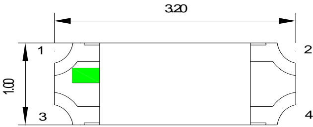
Fig.1-1 Top view
