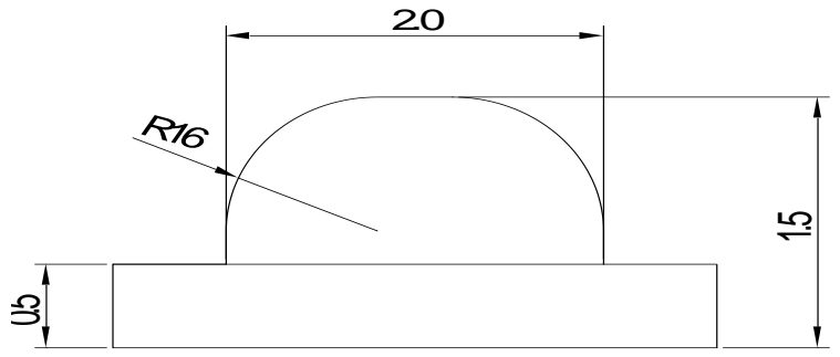
Fig.1-2 Side view
