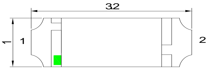
Fig.1-1 Top view
