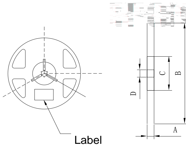
Fig.2-2 Reel Dimension
