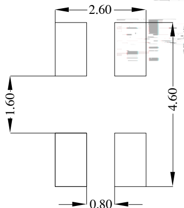
Fig.1-5 Soldering Patterns
