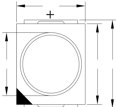
Fig.1-1 Top View
