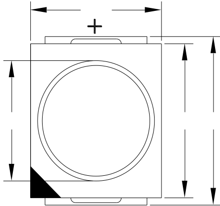
Fig.1-1 Top View
