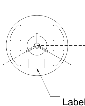
Fig.2-2 Reel Dimension
