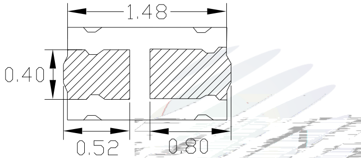
Fig.1-3 Bottom View
