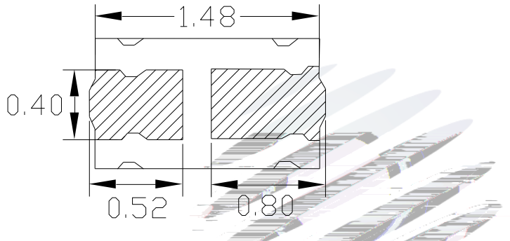
Fig.1-3 Bottom View
