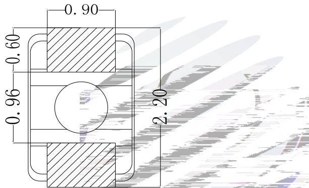
Fig.1-3 Bottom View
